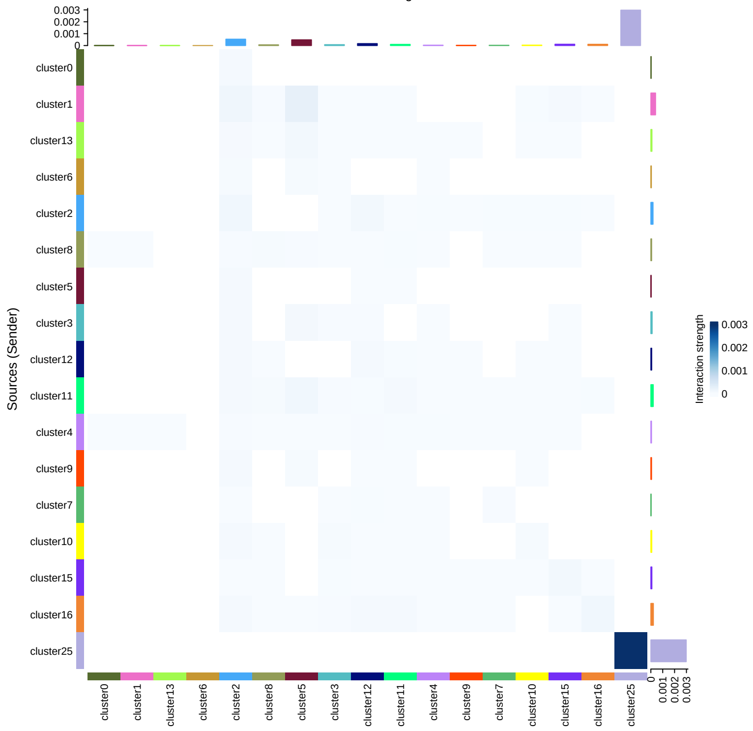
Interaction strength
